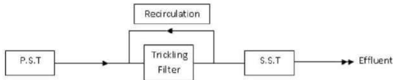
Single Stage High Rate Trickling Filter
