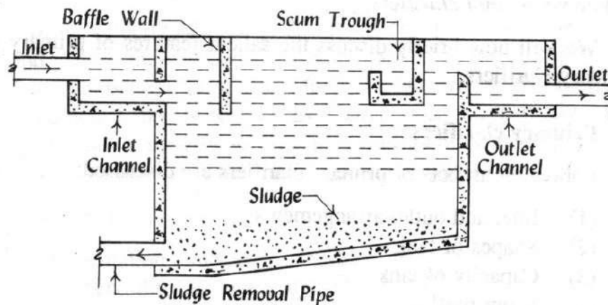
Rectangular settling tank
