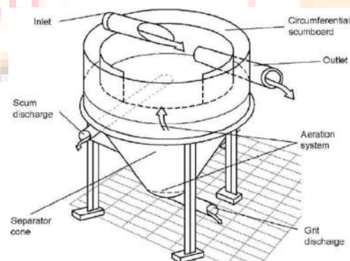
Figure 5.28 Hydraulic regimen of vortex and scum separator
