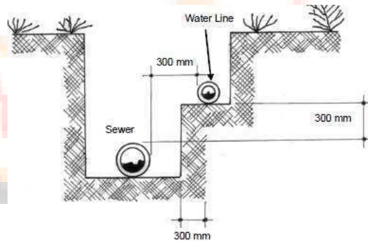
Minimum separation when sewer piping
