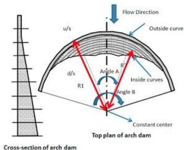
Constant Radii Arch Dam Best suited for U-Shaped Valley
