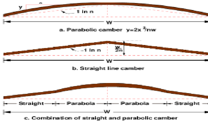
Figure : Different types of camber
