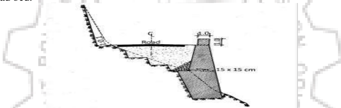
Typical Cross Sections of Embankment with retaining walls
