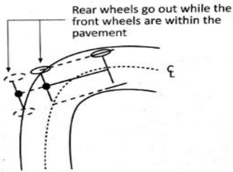
(a) Off-tracking
